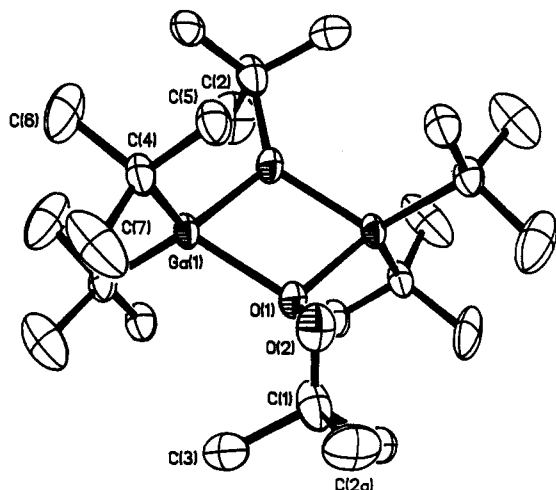
Figure 2. Structure of (^t\text{Bu})_2\text{Ga}(\mu\text{-O}^t\text{Bu})(\mu\text{-OO}^t\text{Bu})\text{Ga}(^t\text{Bu})_2 (8). Thermal ellipsoids are drawn at the 30% level, and hydrogen atoms are omitted for clarity.
