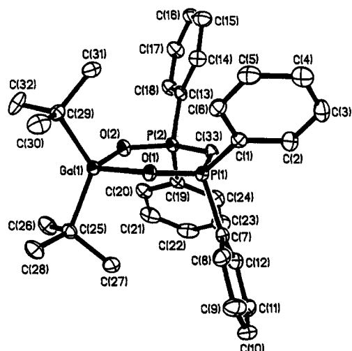
Figure 4. Structure of one of the independent molecules of (t\text{Bu})_2\text{Ga}[(\text{O})\text{P}(\text{Ph})_2\text{CH}(\text{O})\text{P}(\text{Ph})_2] (9). Thermal ellipsoids are drawn at the 40% level, and hydrogen atoms are omitted for clarity.
