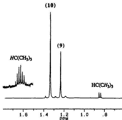
Figure 5. ^1\text{H} NMR showing the formation of (\text{tBu})_2\text{Ga}[(\text{O})\text{P}(\text{Ph})_2\text{CH}(\text{O})\text{P}(\text{Ph})_2] (9) and \text{HC}(\text{CH}_3)_3 as the only products from the thermolysis of \text{Ga}(\text{tBu})_3(\text{dppmO}_2) (10).
